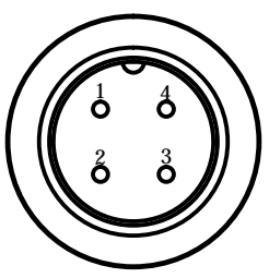
VIEW A 4 PIN FEMALE CONNECTOR
