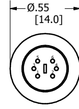
VIEW B 6 PIN MALE CONNECTOR
