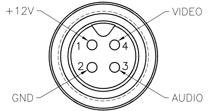
VIEW A 4 PIN MALE PLUG
